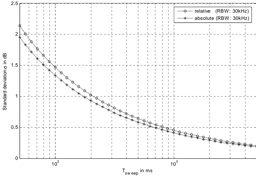
Figure 1: Standard deviation \sigma of spectrum emission mask measurement as a function of sweep time ( T_{sweep} )
